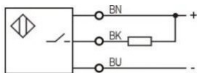
NPN NO
