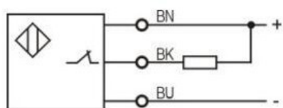
NPN NC
