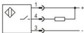
NPN NO
