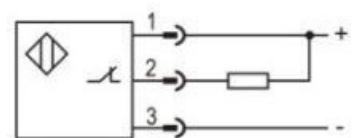
NPN NC
