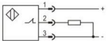
PNP NC
