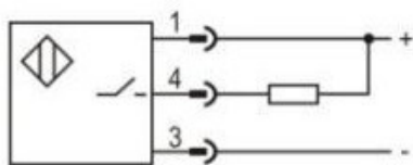
NPN NO
