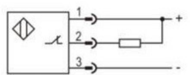
NPN NC
