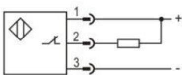
NPN NC
