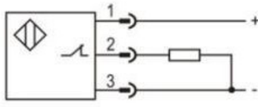
PNP NC
