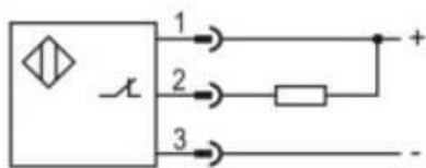
NPN NC
