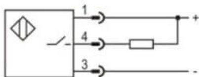
NPN NO
