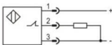
PNP NC
