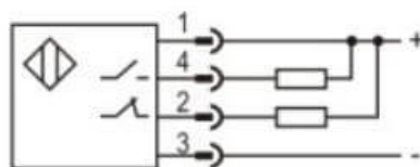
NPN NO+NC
