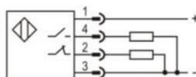
PNP NO+NC
