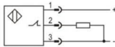
PNP NC
