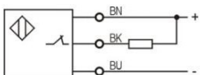
NPN NC
