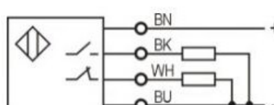
PNP NO+NC
