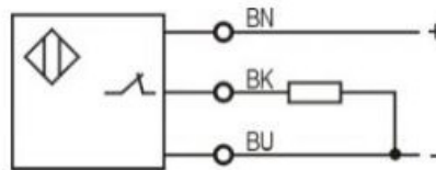
PNP NC
