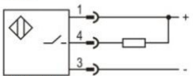
NPN NO
