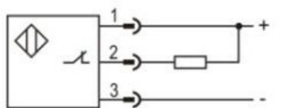
NPN NC
