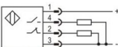
PNP NO+NC
