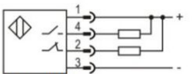
NPN NO+NC
