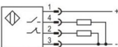
PNP NO+NC
