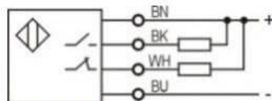
NPN NO+NC
