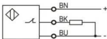
PNP NC
