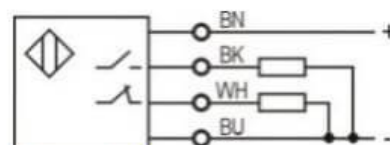
PNP NO+NC
