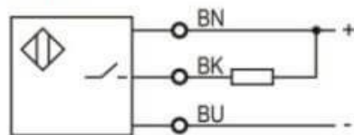
NPN NO
