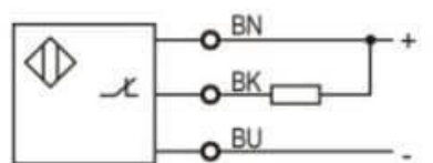
NPN NC
