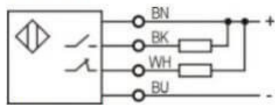
NPN NO+NC
