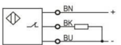
PNP NC
