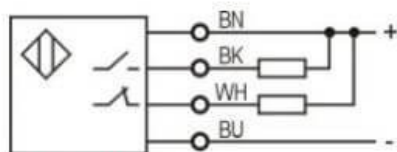
NPN NO+NC
