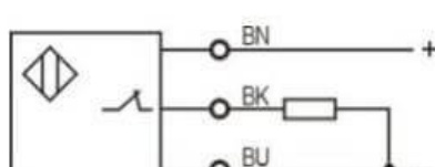
PNP NC
