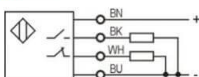
PNP NO+NC
