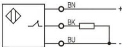
PNP NC
