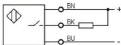
NPN NO
