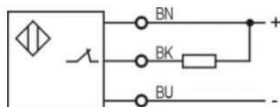
NPN NC
